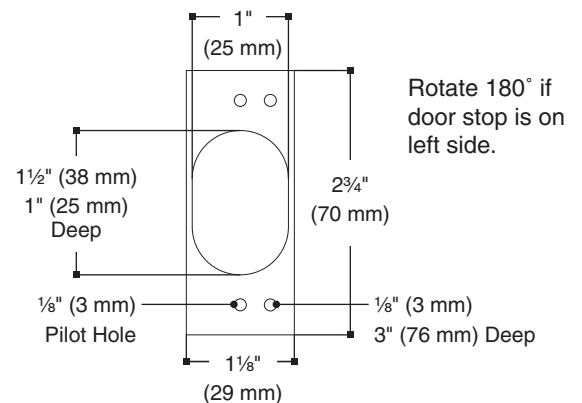
Strike Cut-Out (not to scale)
